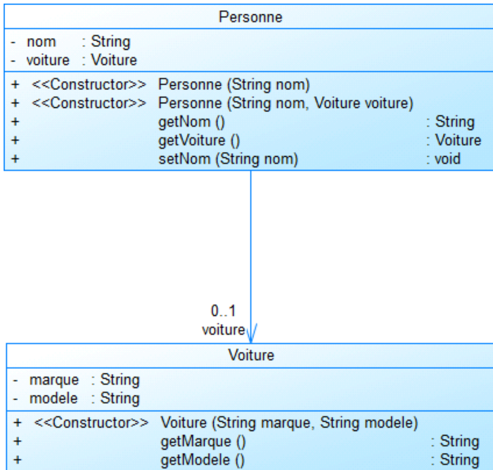
Figure 2.2. Association simple
