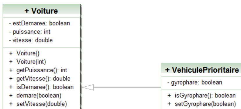
Figure 1.9. Héritage
