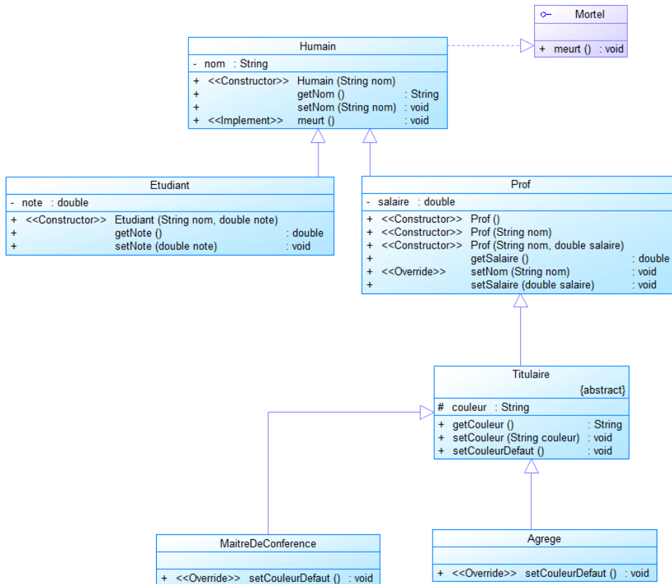
Figure 2.7. Interface
